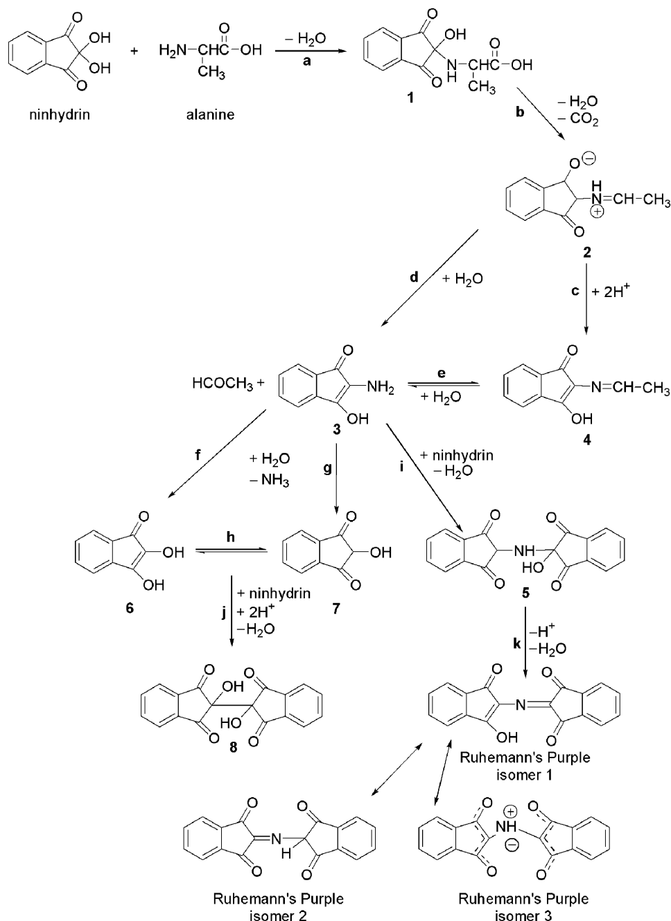
FIG. 4—McCaldin mechanism.
